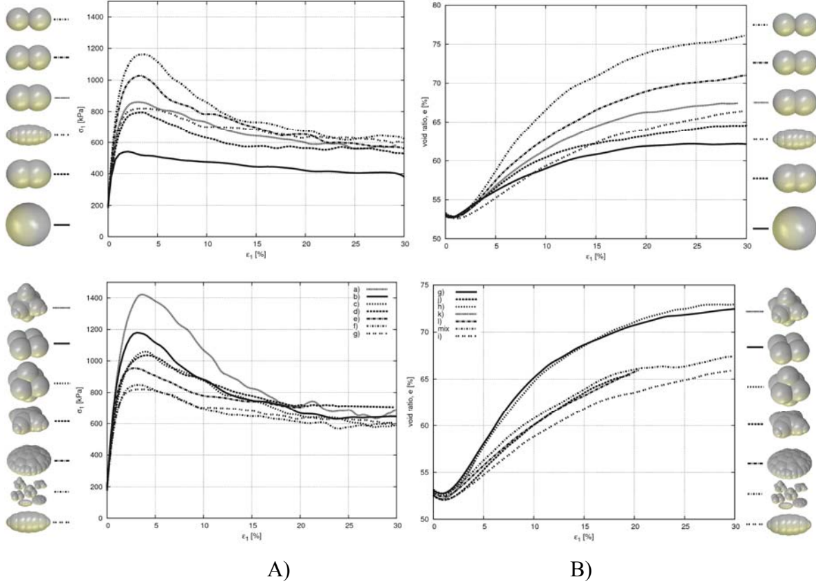
FIGURE 3: Effect of particle roughness (without contact moments) on vertical normal stress \sigma_l versus vertical normal strain \varepsilon_l (A) and volumetric strain e versus vertical normal strain \varepsilon_l (B) during homogeneous triaxial compression test for different grain shapes of Fig.4 ( e_o=0.53 , p=200 kPa, d_{50}=5 mm)
