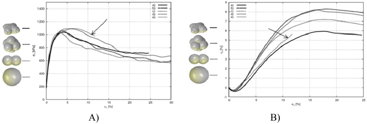
FIGURE 4: Effect of some clusters of spheres of Fig.2 without contact moments and single spheres with contact moments on vertical normal stress \sigma_v versus vertical normal strain \epsilon_v (A) and volumetric strain \epsilon_v versus vertical normal strain \epsilon_v (B) compared to experiments ( \rightarrow ) during homogeneous triaxial compression test ( e_o=0.53 , p=200 kPa, d_{50}=5 mm)
